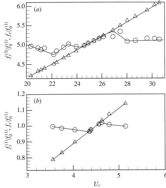
FIGURE 18. Variation of the system's natural frequency ( \circ ) and the vortex shedding frequency ( \triangle ) with U_r around resonance: (a) f_y^{(3)} and f_s ; (b) f_y^{(1)} and f_s . Cylinder 1, T/d = 3.00 . The solid line indicates the trend.
