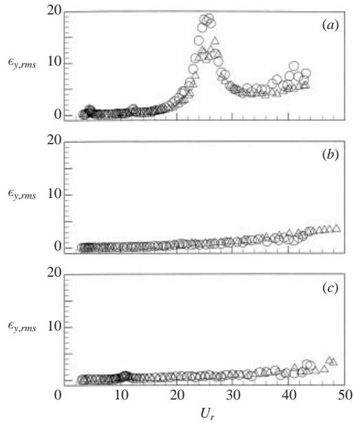
FIGURE 11. Variation of \epsilon_{y,rms} with U_r at various spacing ratios: (a) T/d = 3.00 ; (b) 1.70; (c) 1.13. \circ , Cylinder 1; \triangle , Cylinder 2.
