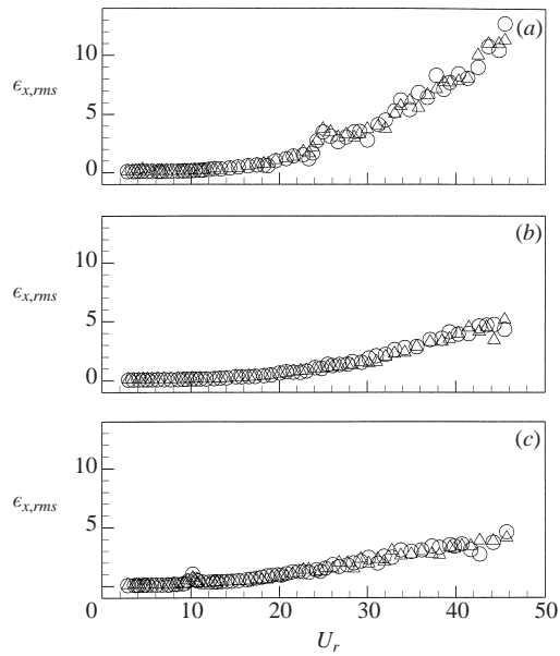
FIGURE 12. Variation of \epsilon_{x,rms} with U_r at various spacing ratios: (a) T/d = 3.00 ; (b) 1.70; (c) 1.13. \circ , Cylinder 1; \triangle , Cylinder 2.
