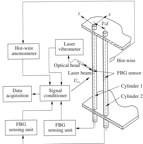
FIGURE 2. Experimental arrangement.
