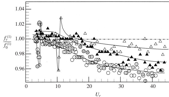
FIGURE 14. Variation of the cross-flow f_y^{(1)} with T/d and U_r . Cylinder 1. \triangle , T/d = 1.13 ; \blacktriangle , 1.70; \circ , 3.00; \bullet , single cylinder; --- , linear model. The solid line indicates the trend.
